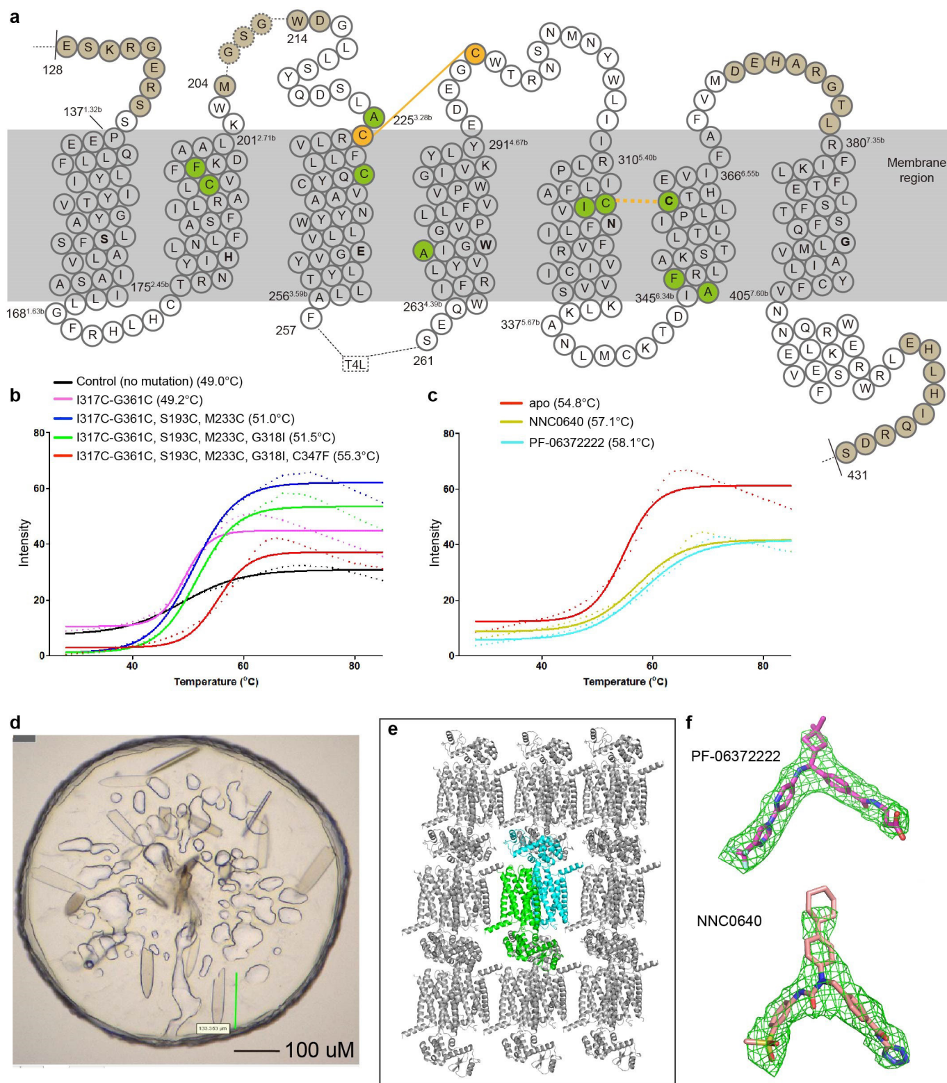
Extended Data Figure 1 | GLP-1R crystallization and structure determination. a , Schematic diagram of GLP-1R TMD construct (residues 128–431). Thermostabilizing mutations (green) are S193C, I196F, S225A, M233C, S271A, I317C, G318I, K346A, C347F and G361C. The single conserved residue among class B GPCRs in each transmembrane helix (designated X.50b in the Wootten residue numbering scheme 16 , in which 'X' is the transmembrane helix number) is indicated in bold. Disordered residues in the structure are shown with a brown background. Engineered ECL1 linker residues are shown as dashed circles. The endogenous and engineered disulfide bonds are shown with solid and dashed orange lines,
