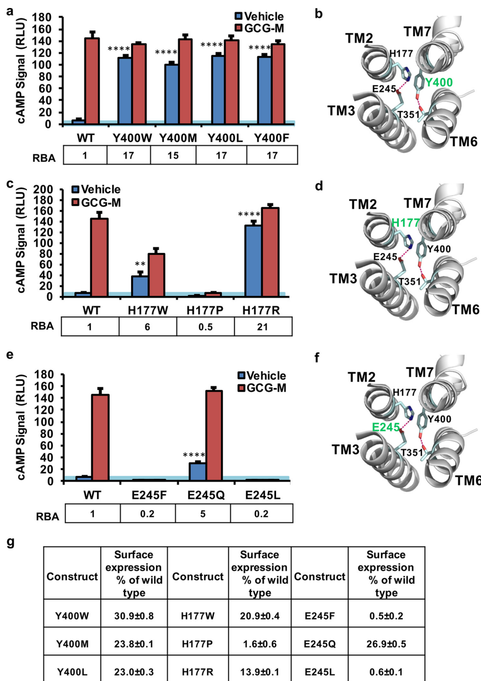
Figure 10. Polar core mutations increase basal GPCR activity. a , c , and e , basal and membrane-tethered GCG-stimulated cAMP signals of GPCR with mutations at position Tyr-400 ( a ), His-177 ( c ), and Glu-245 ( e ). The blue background marks the basal activity of the wild-type full-length GPCR. Relative basal activity (RBA), -fold increase in basal activity of mutant receptors relative to WT receptor. Error bars represent S.D. of triplicate determinations. Two-tailed Student's t test was used to determine p values for data point versus the basal activity of WT GPCR: **, p \leq 0.01 ; ****, p \leq 0.0001 . b , d , and f , structure of the GPCR polar core in which residues Tyr-400 ( b ), His-177 ( d ), and Glu-245 ( f ) are highlighted in green. g , cell surface expression of GPCR with substitutions at position Tyr-400, His-177, and Glu-245. Data are presented as percent expression levels relative to that of WT receptor (100%). RLU, relative luciferase unit, which is the ratio of the CRE-luciferase activity to the Renilla luciferase activity.
